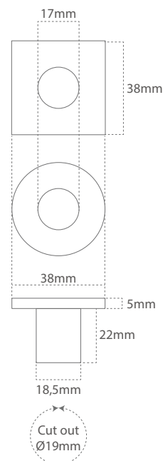
Mounting bracket
