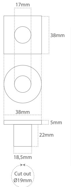
Mounting bracket
